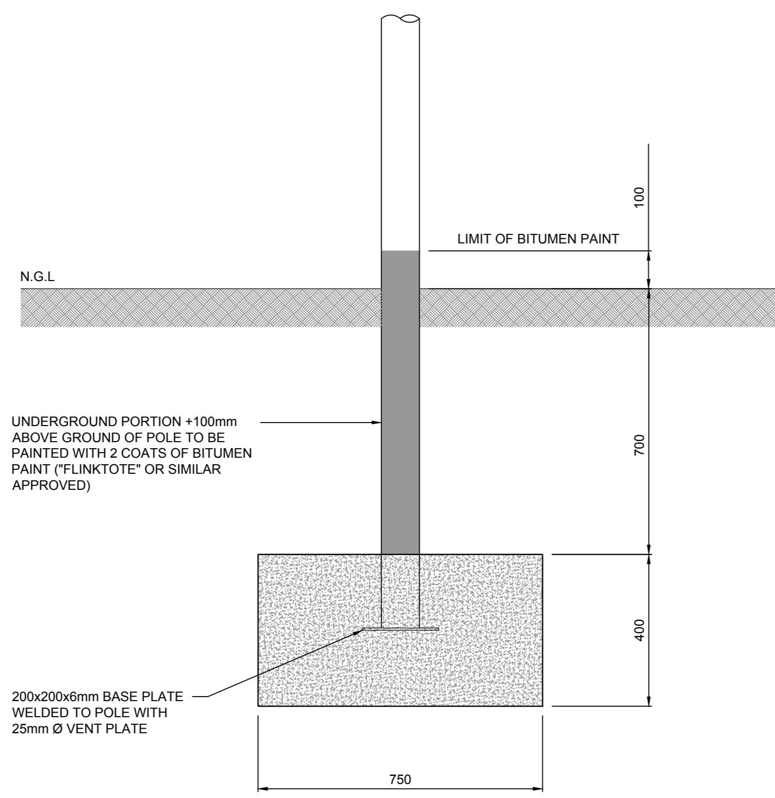
SECTION THROUGH POLE AND FOOTING SCALE 1:10
