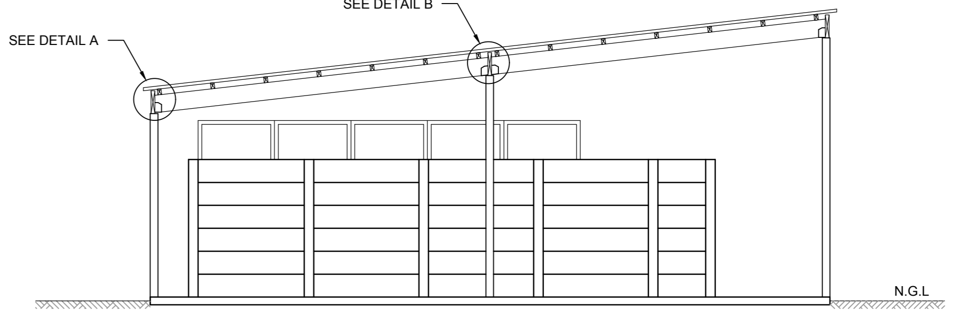
SIDE ELEVATION SCALE 1:50
