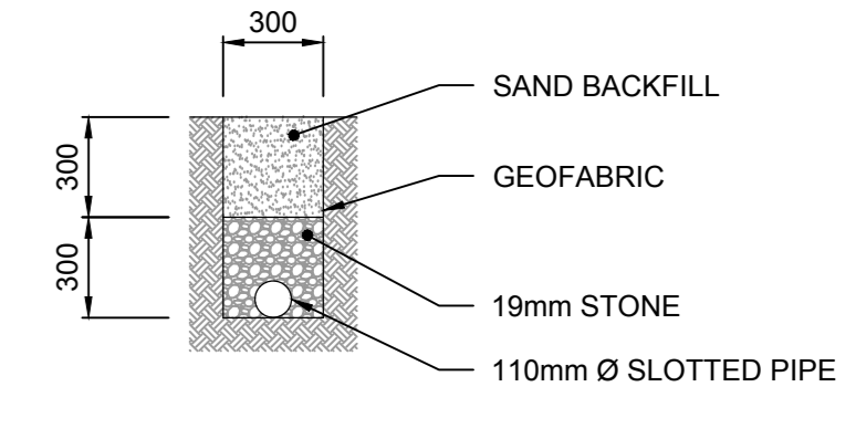
SUBSOIL DRAIN SCALE 1:25
