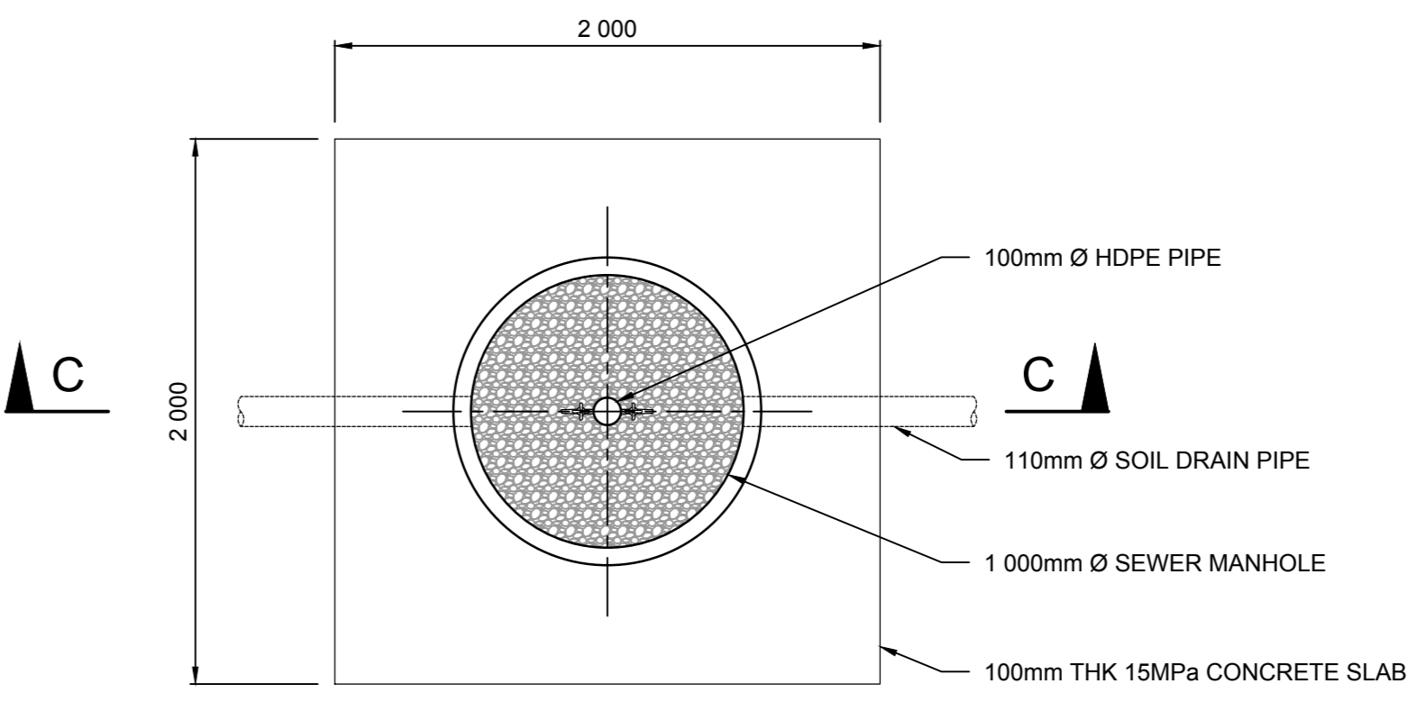
STAND PIPE DETAIL SCALE 1:25
