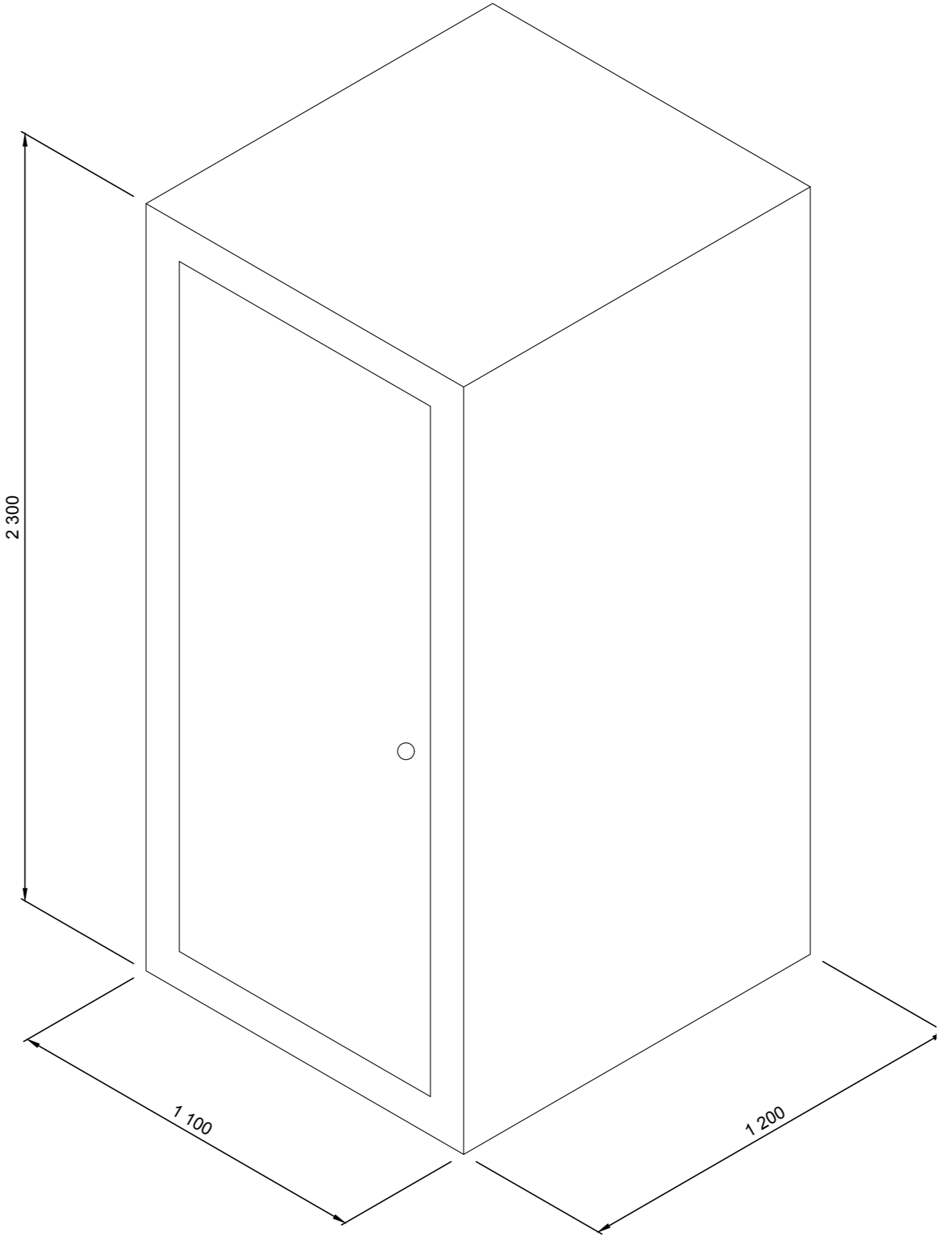
TYPICAL CHEMICAL TOILET SCALE 1:15
